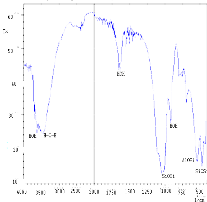
Figure-2. IR spectrum for Iliri clay leached in 25% acid
