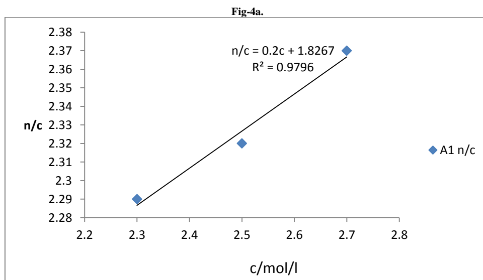
Figures-4a-4h. Representative plot of n/c versus c for adsorption of 1-aminobutane on Iliri clays
