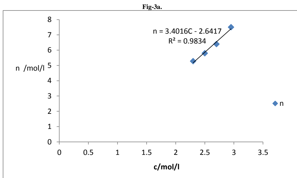
Figure-3. Representative Langmuir adsorption isotherms for 1-aminobutane on different Iliri clays
