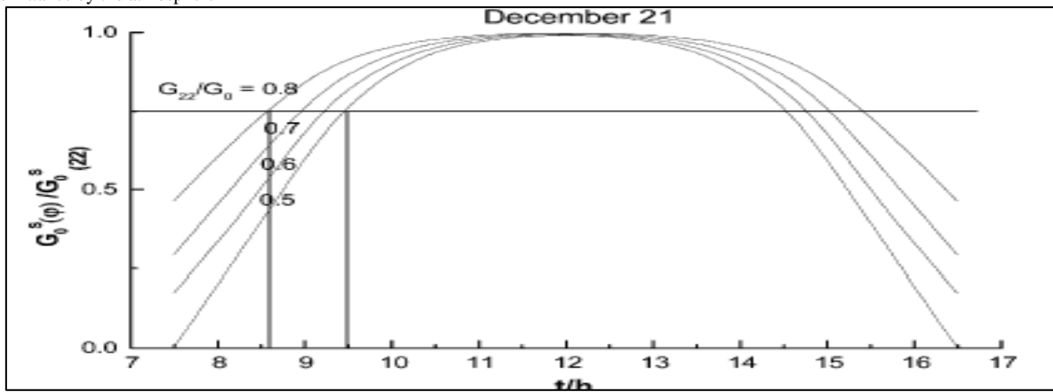
Figure-7. Calculated values of normal irradiance by solar rays relative to the values obtained at the apex on December 21 for different transmittance by the atmosphere
