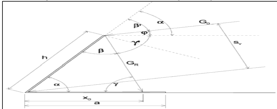
Figure-3. Schematic representation of the reflection of a sunbeam to the ground of a greenhouse with a reflecting wall
