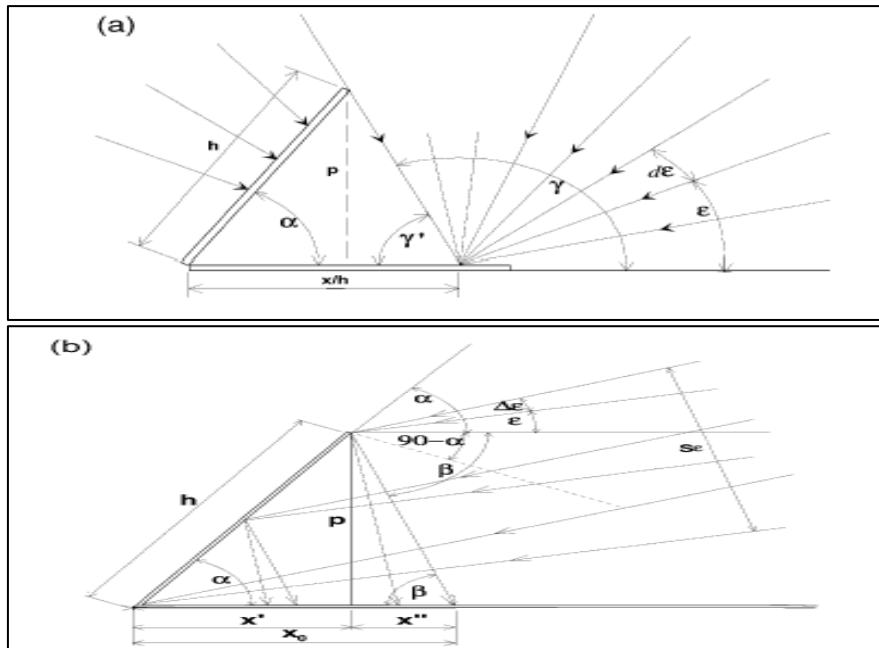
Figure-5. Schematic representations of (a) diffuse light falling onto a point at distance x/h from the reflecting wall, and of (b) diffuse light reflected by the wall
