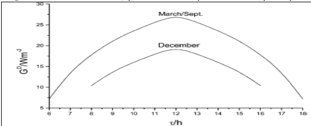
Figure-12. Ground irradiance from diffuse (sky) radiation from a clear sky at the shortest winter day and at equinox
