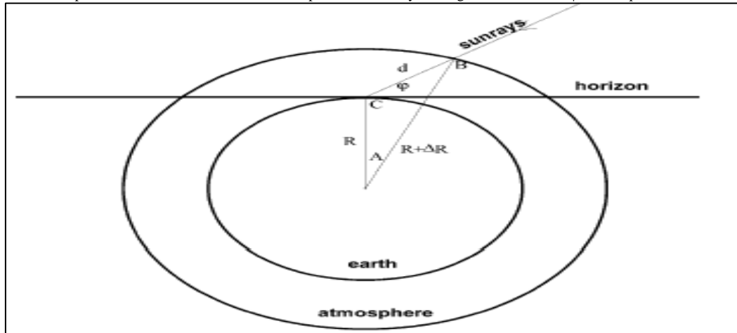
Figure-6. Schematic representations of the earth and its atmosphere with sunrays falling at an inclination \varphi with respect to the horizon
