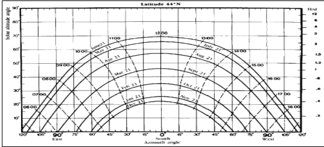
Figure-8. Dependence of the elevation and azimuth angle of the sun on the time of a day at different days of a year at NL 44° [34]
