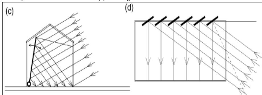
Figure-2. Greenhouse types according to the applied mode of reflection of solar radiation: (a) fixed vertical reflecting wall (b) fixed inclined reflecting wall (c) reflecting wall with variable inclination (d) reflecting wall with louvers
