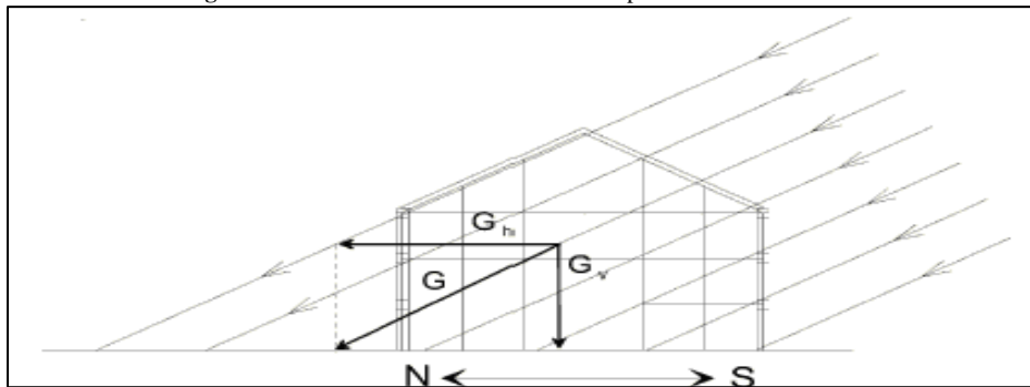
Figure-1. Relative horizontal and vertical components of solar radiation
