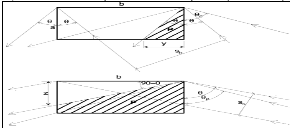
Figure-4. Influence of the azimuth angle \theta \neq 0 on the effectiveness of exposure of the ground to reflected light
