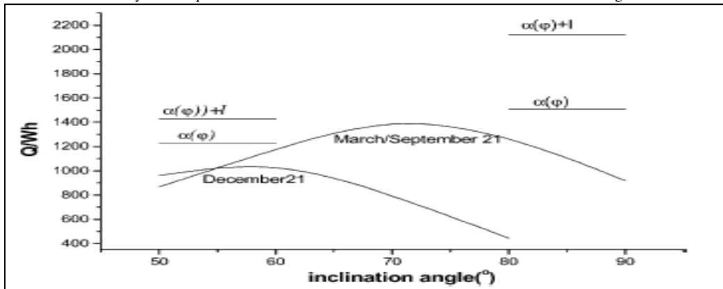
Figure-11. Dependence of the daily energy gain in different types of greenhouses. Different types illustrate the effects of the inclination angle of the wall at the shortest winter day and at equinox. The horizontal lines show the effects of different inclination angles without and with louvers
