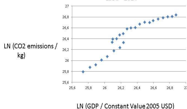
Figure 6. Indonesia: GDP-CO 2 link: y = 0,95x + 1,58 ; R^2 = 0,89 GDP-CO 2 emissions Indonesia 1990 - 2014
