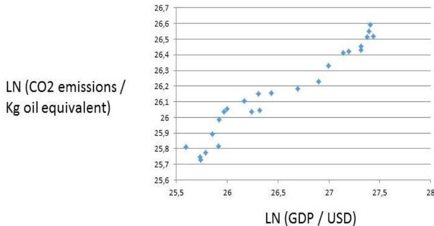
Figure-9. Turkey GDP=CO2 link: y = 0,41x ; R^2 = 0,95 GDP – CO2 Emissions Turkey 1990 - 2014
