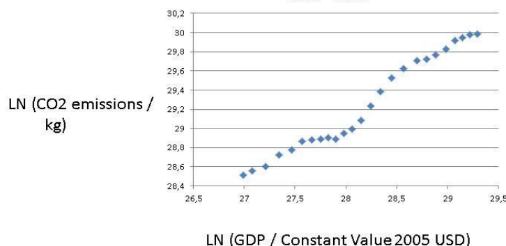
Figure-2. CHINA: GDP-CO2 link: y = 0,70x ; R^2 = 0,97
