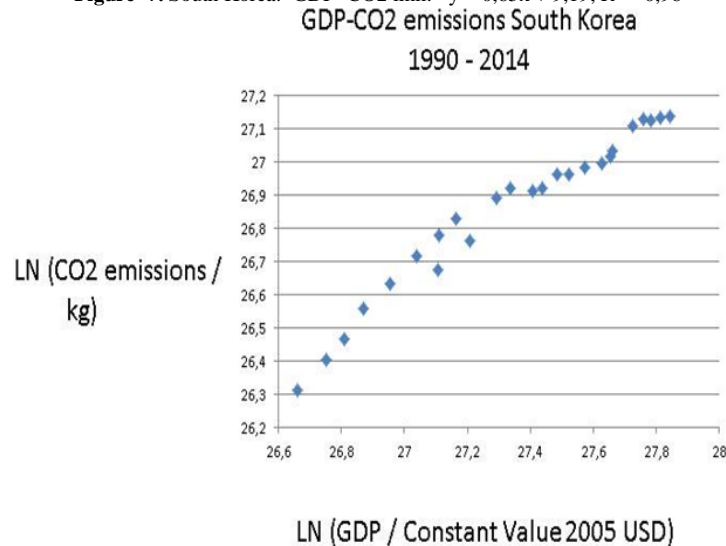
Figure -7. South Korea: GDP=CO2 link: y = 0,65x + 9,19 ; R^2 = 0,96
