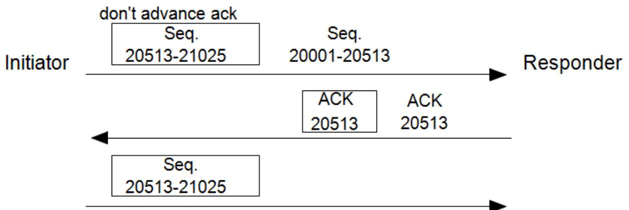
Figure-3. Retransmission Test
